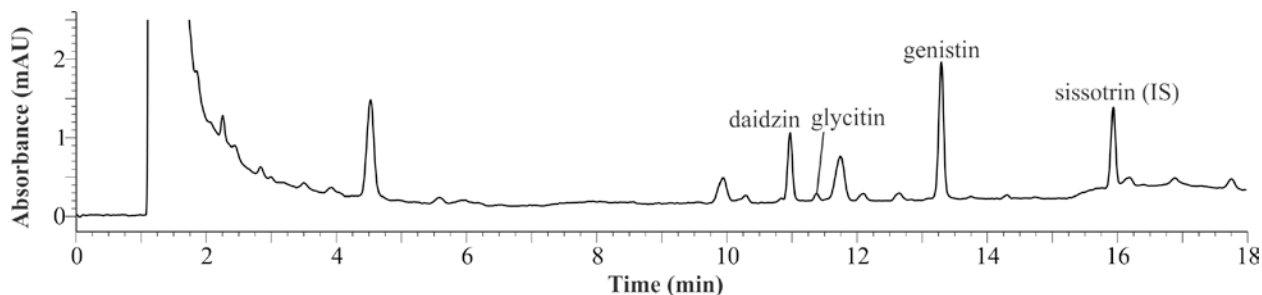
Figure 2. Chromatogram showing separation and detection of isoflavones in SRM 3237 using LC/absorbance. For this method, an Ascentis Express RP-Amide column (150 mm \times 4.6 mm, 2.7 \mu m particle size; Supelco, Bellefonte, PA, USA) was held at 35 ^{\circ} C. The separation was performed using a gradient consisting of 5 mmol/L ammonium acetate in water and acetonitrile. Absorbance detection was utilized at 254 nm.
