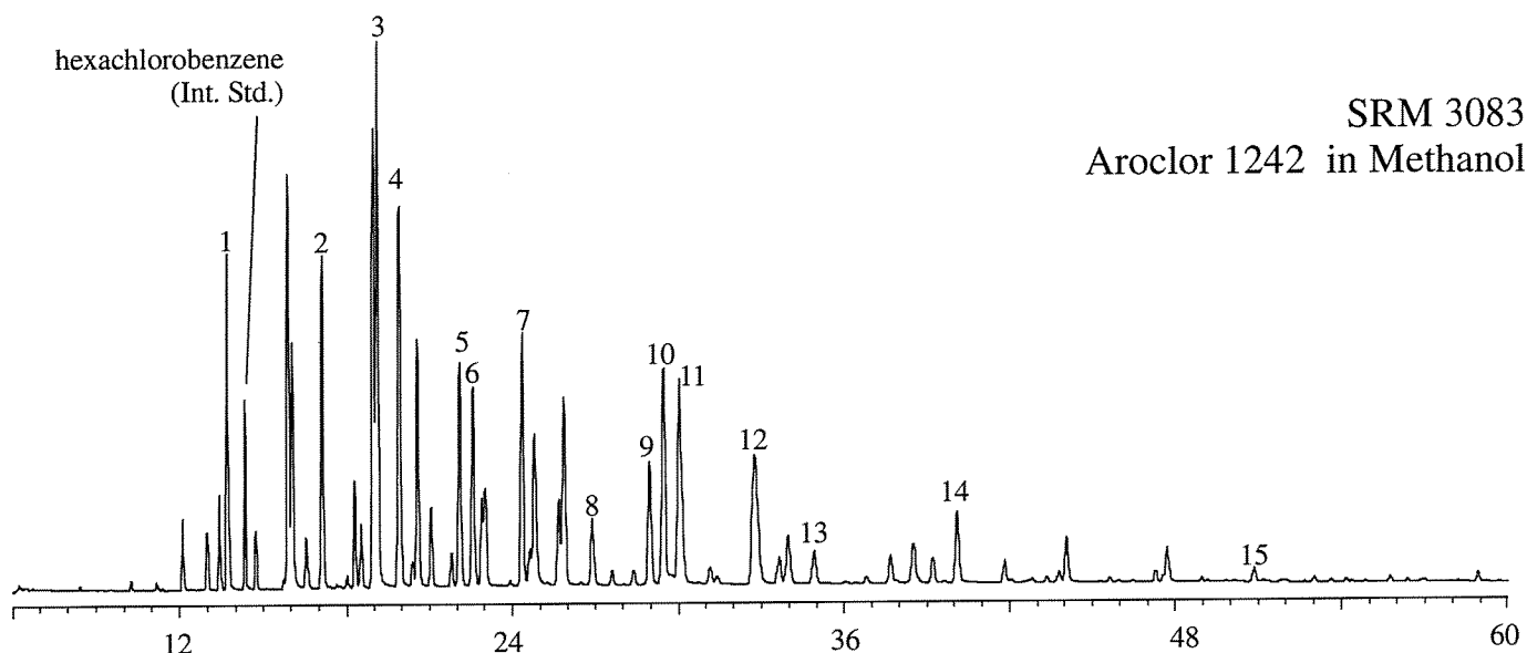
Figure 1. Gas chromatograms from the analysis of aroclors in methanol. The peaks used for quantification of the Aroclor mass in each solution are shown. (Int. Std.) = internal standard, x-axis represents "time" in minutes
