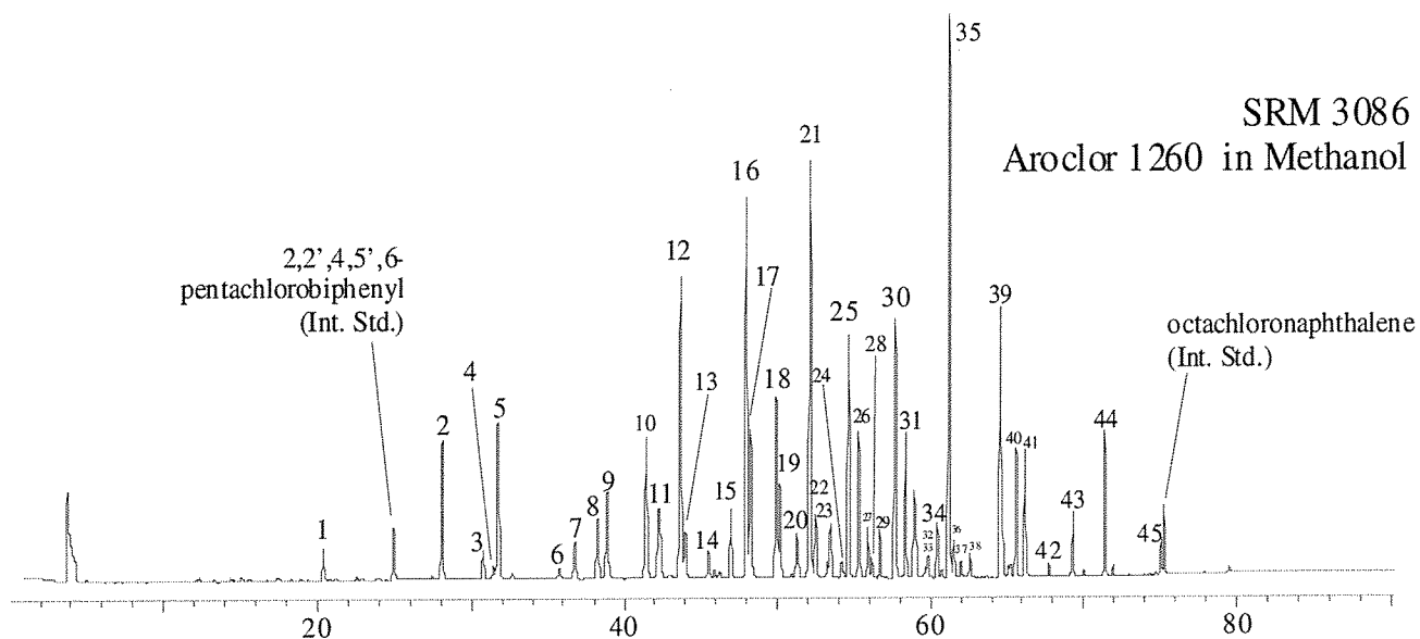
Figure 1, continued. Gas chromatograms from the analysis of aroclors in methanol. The peaks used for quantification of the Aroclor mass in each solution are shown. (Int. Std.) = internal standard, x-axis represents "time" in minutes
