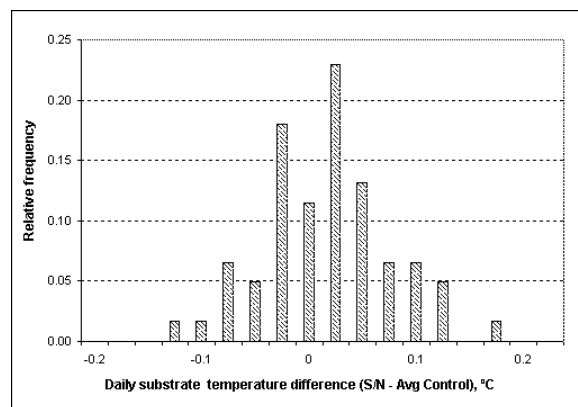
Figure 7. Histogram of the daily substrate temperature difference between calibrations and control measurements. The mean difference is 0.005^{\circ}\text{C} , and the standard deviation is 0.06^{\circ}\text{C} .
