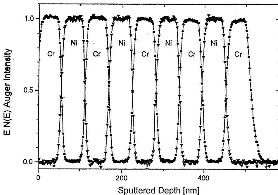
Figure 2. Auger sputter depth profile representative of SRM 2135c obtained using 1 keV argon ion bombardment. The pure Ni and Cr Auger intensities shown have been normalized.
