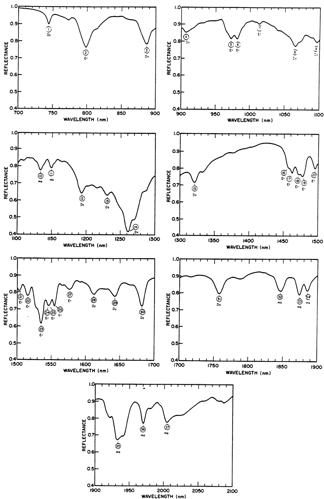
Fig. 2 Reflectance Spectrum of SRM 1920, Near Infrared Reflectance Wavelength Standard.
